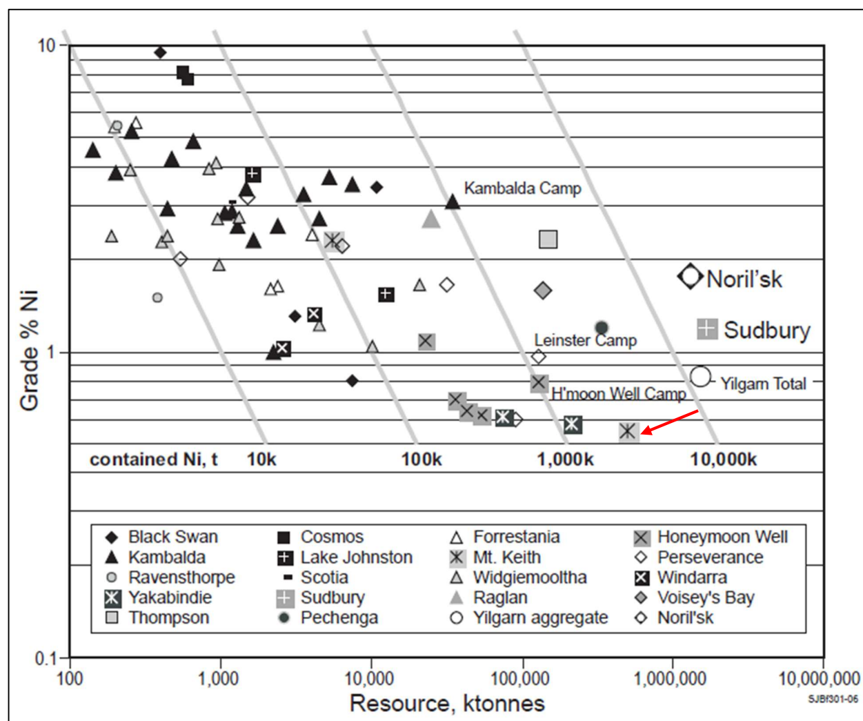
Figure 8-2. Nickel grade and deposit tonnage distribution in traditional magmatic (e.g., Sudbury, Noril'sk, Voisey's Bay) and komatiite-hosted (e.g., Kambalda Camp, Black Swan, Windarra) settings. The Reid Deposit is most like the high-tonnage/low-grade deposits found at Mt. Keith (red arrow) (after Barnes, 2006).
