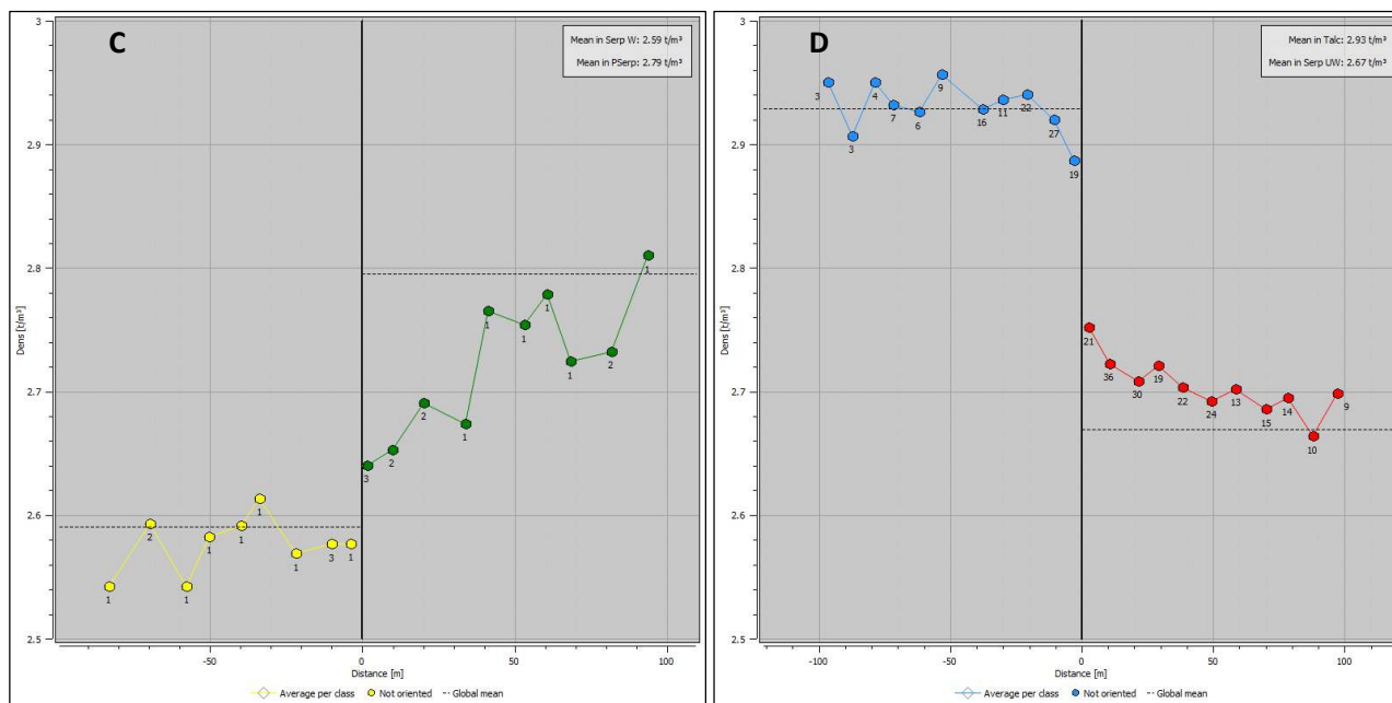
Figure 14-22. Contact analysis plots of density values at: A) Serp W/Serp UW domain boundary, B) Serp UW/PSerp domain boundary, C) Serp W/PSerp domain boundary and D) Talc/Serp UW domain boundary (Caracle Creek, 2026).
