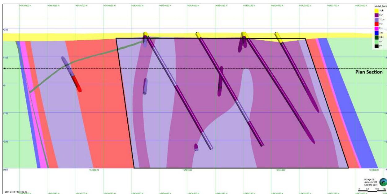
Figure 14-6. Vertical section 457345 mE (Looking East) of the lithology model and drill holes showing lithology intercepts. Some intercepts may not precisely match their corresponding feature due to the 100 m section width. The black box represents the current resource boundary and main modelling area, and the dashed line is the trace of the plan section presented in Figure 14-5 (Caracle Creek, 2026).
