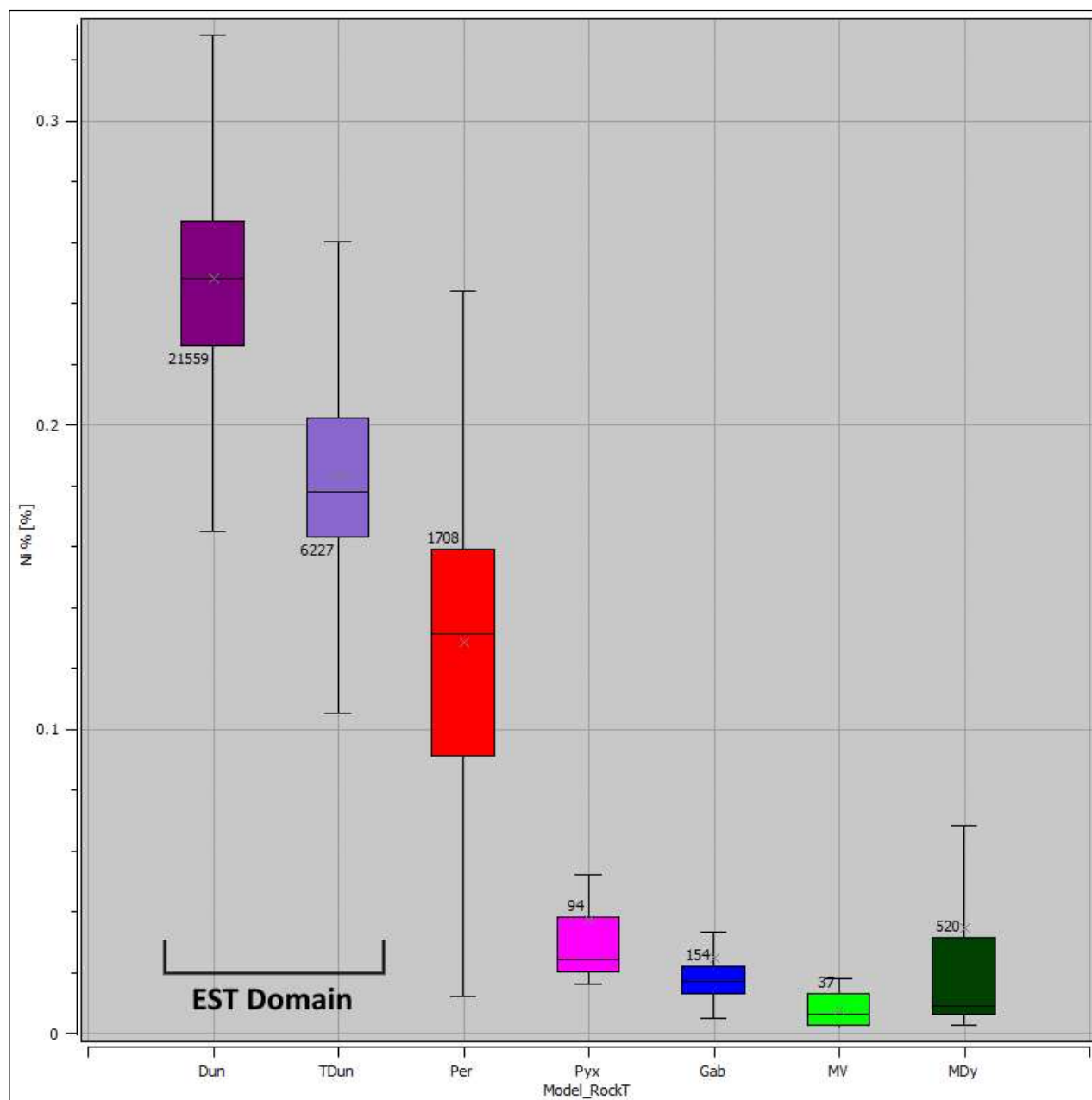
Figure 14-9. Boxplot of nickel grades according to the lithology model (Caracle Creek, 2026).
