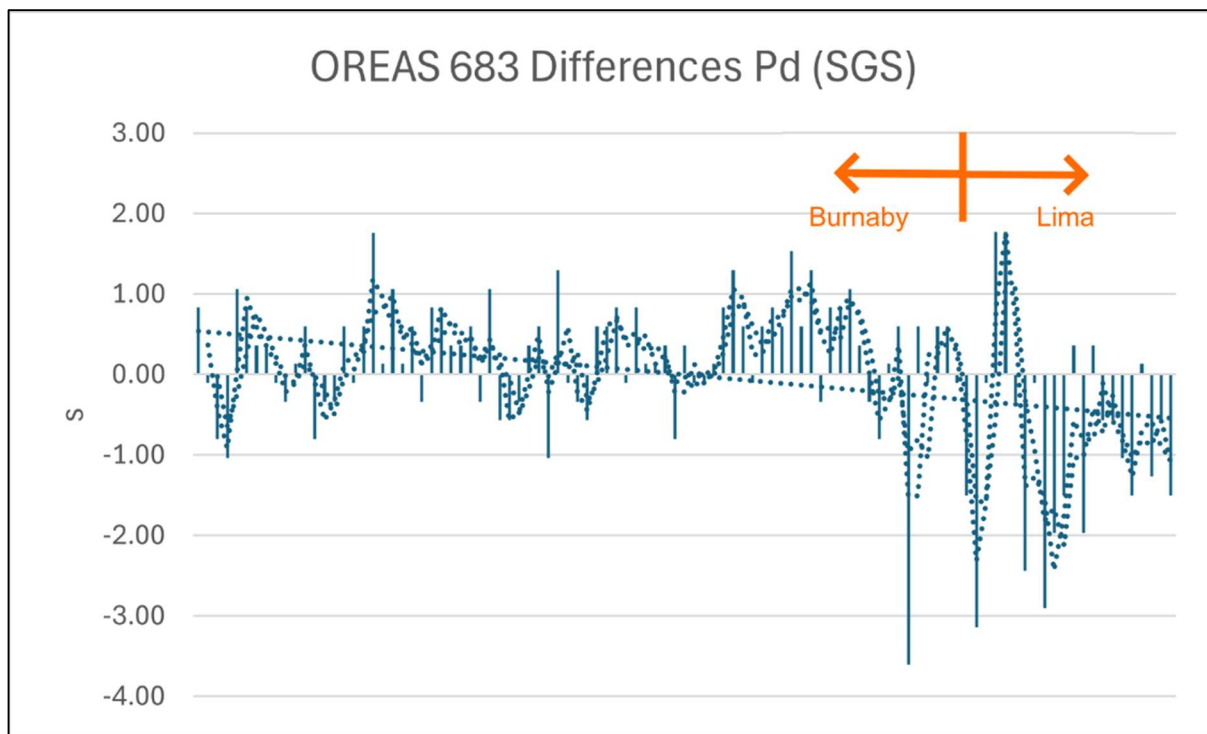
Figure 11-11. CRM OREAS 683 – Number of Standard Deviations Difference for Pd Analysis from the Certified Value for Various Analytical Runs at SGS (Caracle Creek, 2026).
