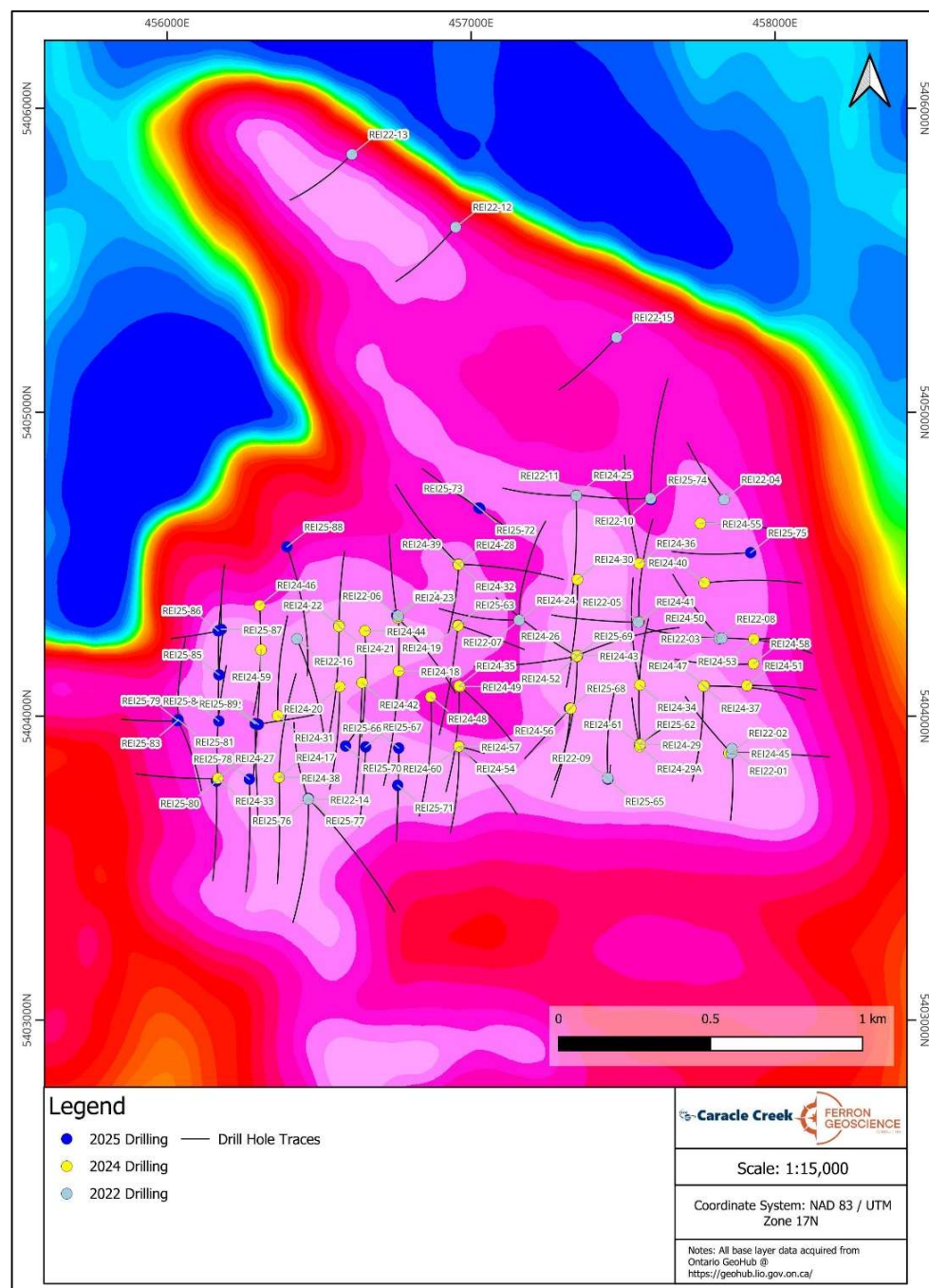
Figure 10-1. Plan map showing the location of the 2022, 2024 and 2025 drill hole collars and traces, Reid Project (Caracle Creek, 2026).
