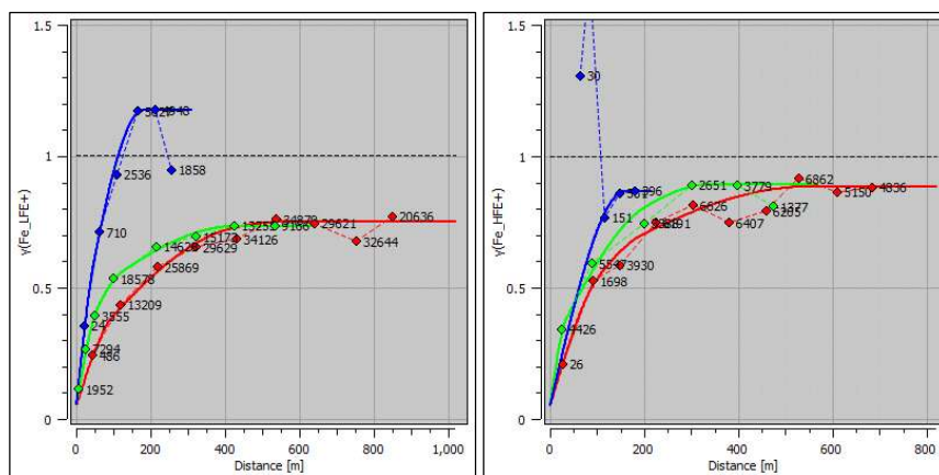
Figure 14-25. Iron variograms for the LFE (left) and HFE (right) domains (Caracle Creek, 2026).
