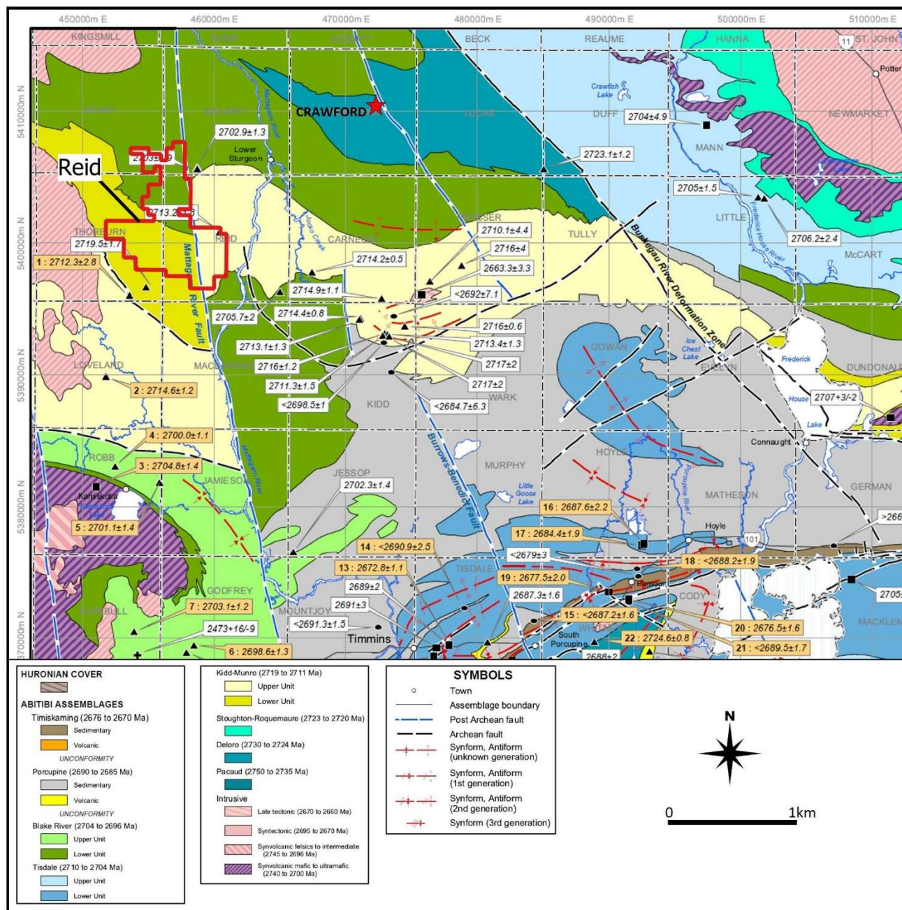
Figure 7-2. Township-scale generalized geology and rock age determinations showing the location of the Reid Nickel Sulphide Project's mining claims boundary (red) and the location of the Crawford Project (red star) to the northeast (after Ayer et al. , 2005).
