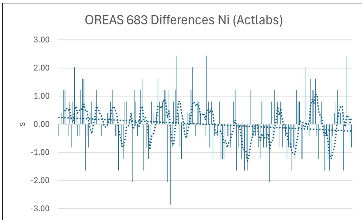
Figure 11-5. CRM OREAS 683 – Number of Standard Deviations Difference for Ni Analysis from the Average Value for Various Analytical Runs at Actlabs (Caracle Creek, 2026).
