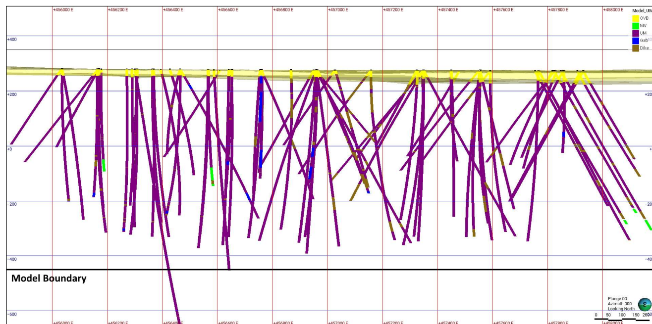
Figure 14-2. Longitudinal view (Looking North) of the Reid Property with the overburden volume (transparent yellow) and CNC drill holes showing the main rock types, including the ultramafic package (UM) coloured in purple (Caracle Creek, 2026).
