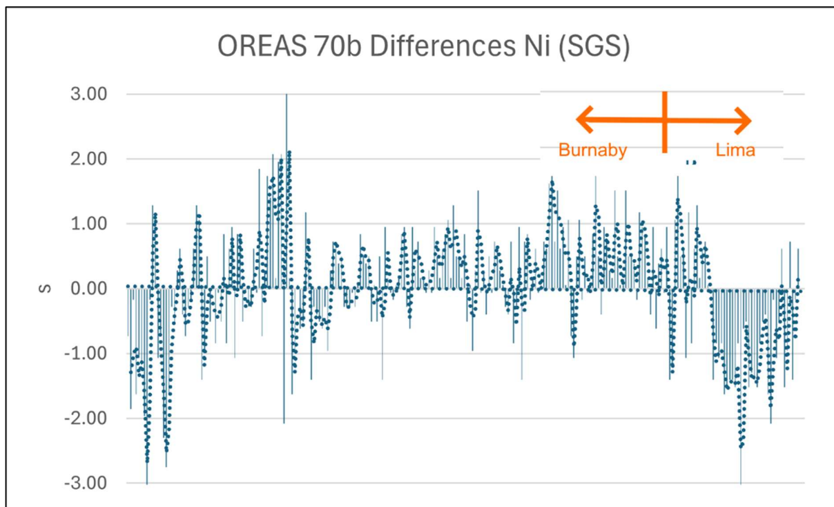
Figure 11-3. CRM OREAS 70b – Number of Standard Deviations Difference for Ni Analysis from the Average Value for Various Analytical Runs at SGS (Caracle Creek, 2026).
