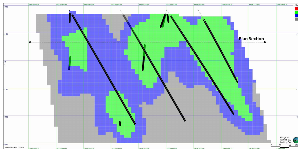
Figure 14-38. Vertical section 457,345 E (Looking East) of the Reid resource classification against drill hole intercepts within the EST domain. Intercepts shown within a 100 m section width. Block colours represent measured (red), indicated (green) and inferred (blue) resource classes, as well as unclassified potential (grey). The dashed line is the trace of the plan section presented in Figure 14-37 (Caracle Creek, 2026).
