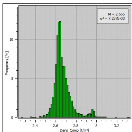
Figure 14-16. Histogram of density values within the EST Domain (Caracle Creek, 2026).
