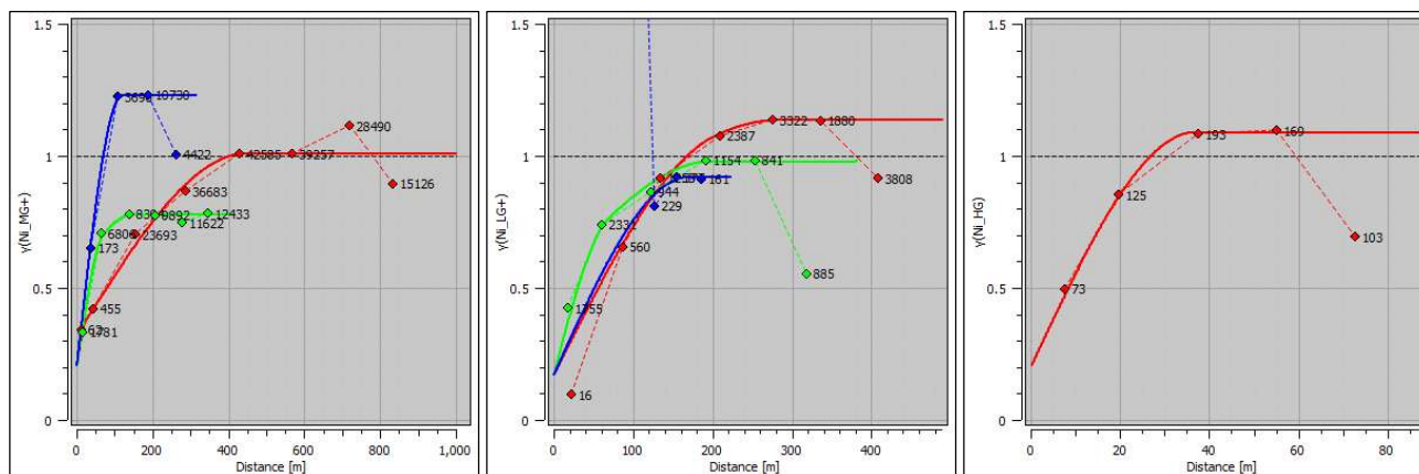
Figure 14-23. Nickel variograms for the MG (left), LG (centre) and HG (right) domains (Caracle Creek, 2026).
