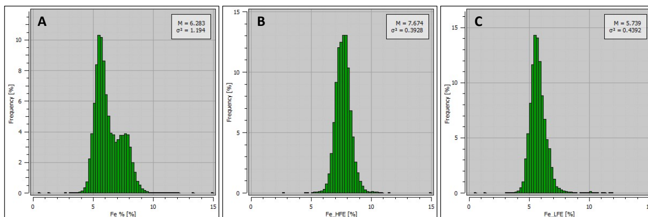
Figure 14-13. Iron grade histograms within: A) EST Domain, B) HFE Domain and C) LFE domain (Caracle Creek, 2026).
