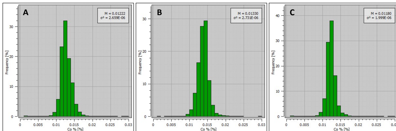
Figure 14-14. Cobalt grade histograms within: A) EST Domain, B) HFE Domain and C) LFE domain (Caracle Creek, 2026).
