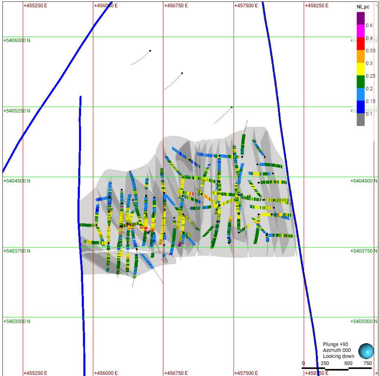
Figure 14-10. Plan view of the EST domain (transparent grey), major faults (blue lines) and nickel grade drill hole intervals (Caracle Creek, 2026).
