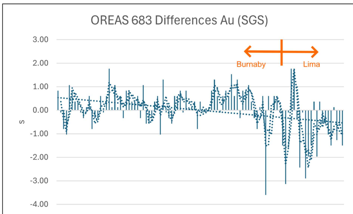
Figure 11-10. CRM OREAS 683 – Distribution of Standard Deviations Difference for Au Analysis from the Average Value for Various Analytical Runs at SGS (Caracle Creek, 2026).
