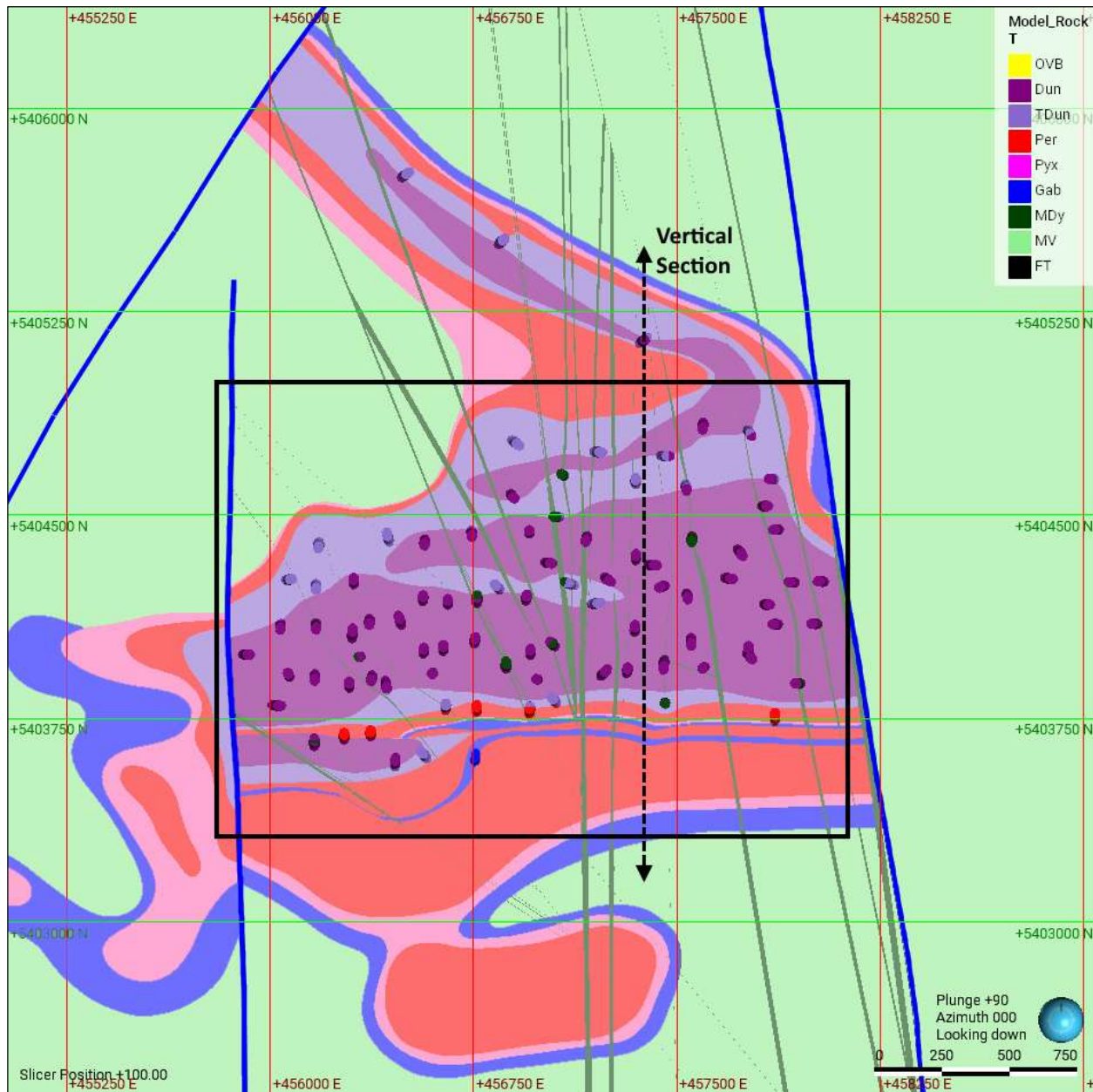
Figure 14-5. Plan section (RL 100) of the Reid lithology model, major faults (blue lines) and coded drill hole intervals. The black rectangle represents the resource boundary and main modelling area, and the dashed line is the trace of the vertical section presented in Figure 14-6 (Caracle Creek, 2026).
