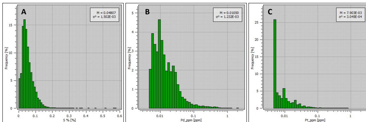
Figure 14-15. Histograms within the EST Domain for: A) Sulphur, B) Palladium and C) Platinum (Caracle Creek, 2026).
