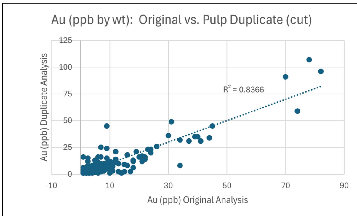
Figure 11-15. Plot of Absolute Concentrations (capped) of Pairs of Duplicate Samples Analyzed for Au (Caracle Creek, 2026).
