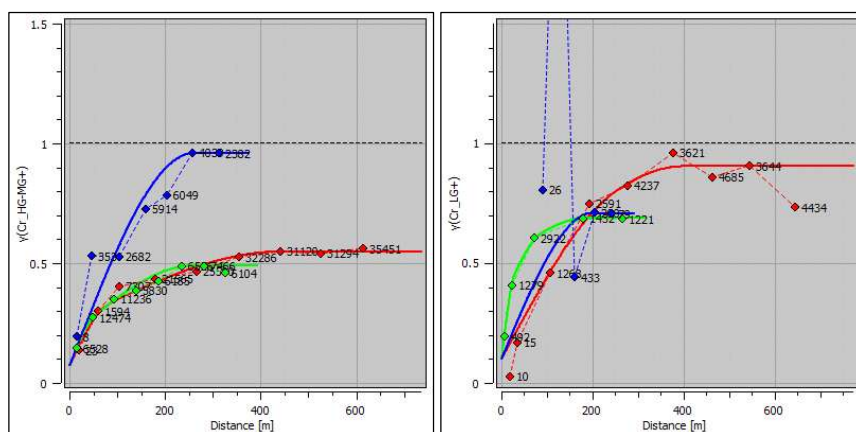
Figure 14-26. Chromium variograms for the HG+MG (left) and LG (right) domains (Caracle Creek, 2026).
