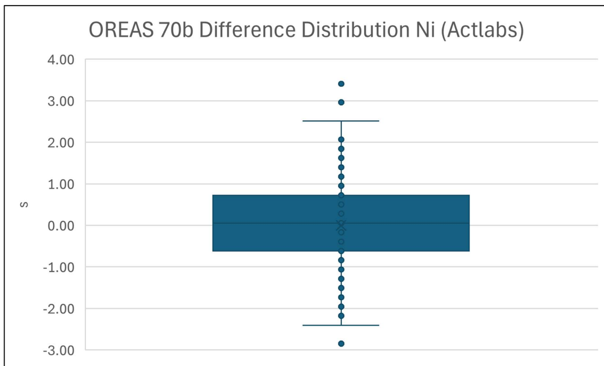
Figure 11-2. CRM OREAS 70b – Distribution of Standard Deviations Difference for Ni Analysis from the Average Value at Actlabs (Caracle Creek, 2026).
