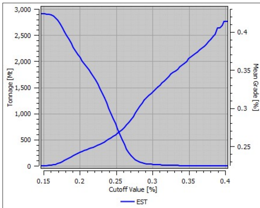
Figure 14-40. Nickel grade-tonnage curve for the pit-constrained Reid Deposit. Not equivalent to a mineral resource statement as by necessity it comprises all mineralized blocks above the pit, regardless of class (Caracle Creek, 2026).
