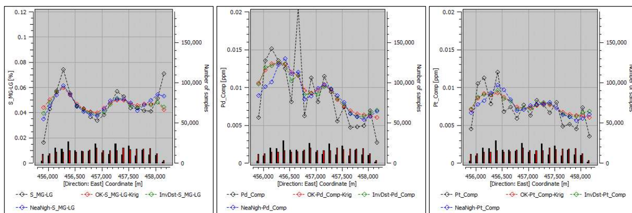
Figure 14-35. Swath plots of sulphur (left) for validation of the MG+LG domain, and of palladium (centre) and platinum (right) for validation of the EST domain (Caracle Creek, 2026).
