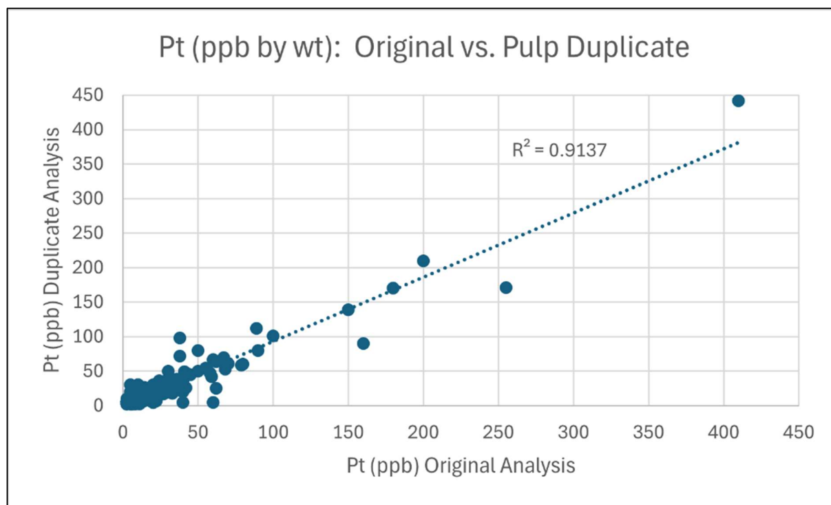
Figure 11-16. Plot of Absolute Concentrations of Pairs of Duplicate Samples Analyzed for Pt (Caracle Creek, 2026).
