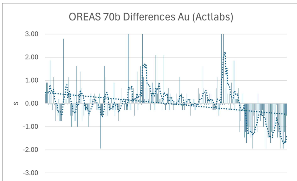
Figure 11-9. CRM OREAS 70b – Number of Standard Deviations Difference for Au Analysis from the Average Value for Various Analytical Runs at Actlabs (Caracle Creek, 2026).
