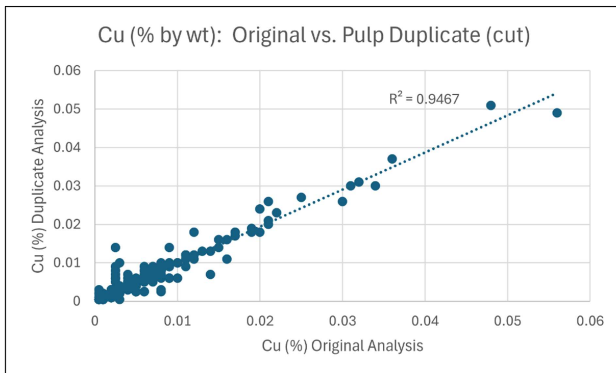
Figure 11-17. Plot of Absolute Concentrations (capped) of Pairs of Duplicate Samples Analyzed for Cu (Caracle Creek, 2026).
