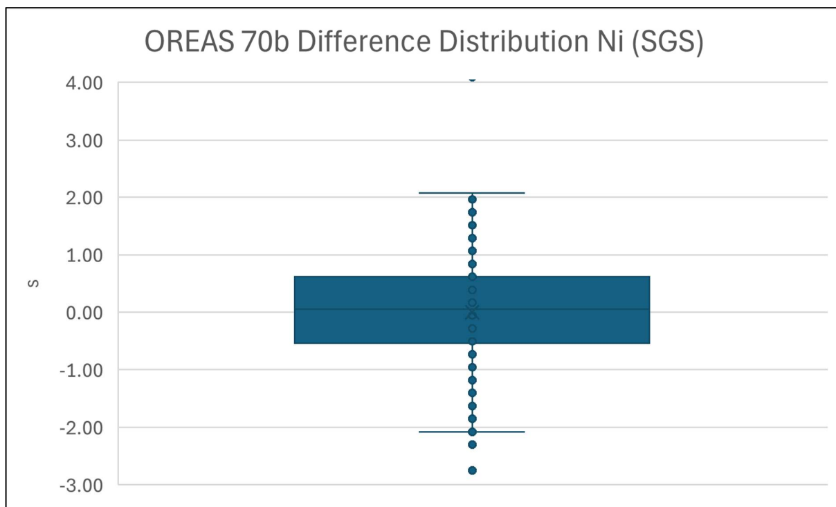
Figure 11-4. CRM OREAS 70b – Distribution of Standard Deviations Difference for Ni Analysis from the Average Value at SGS (Caracle Creek, 2026).
