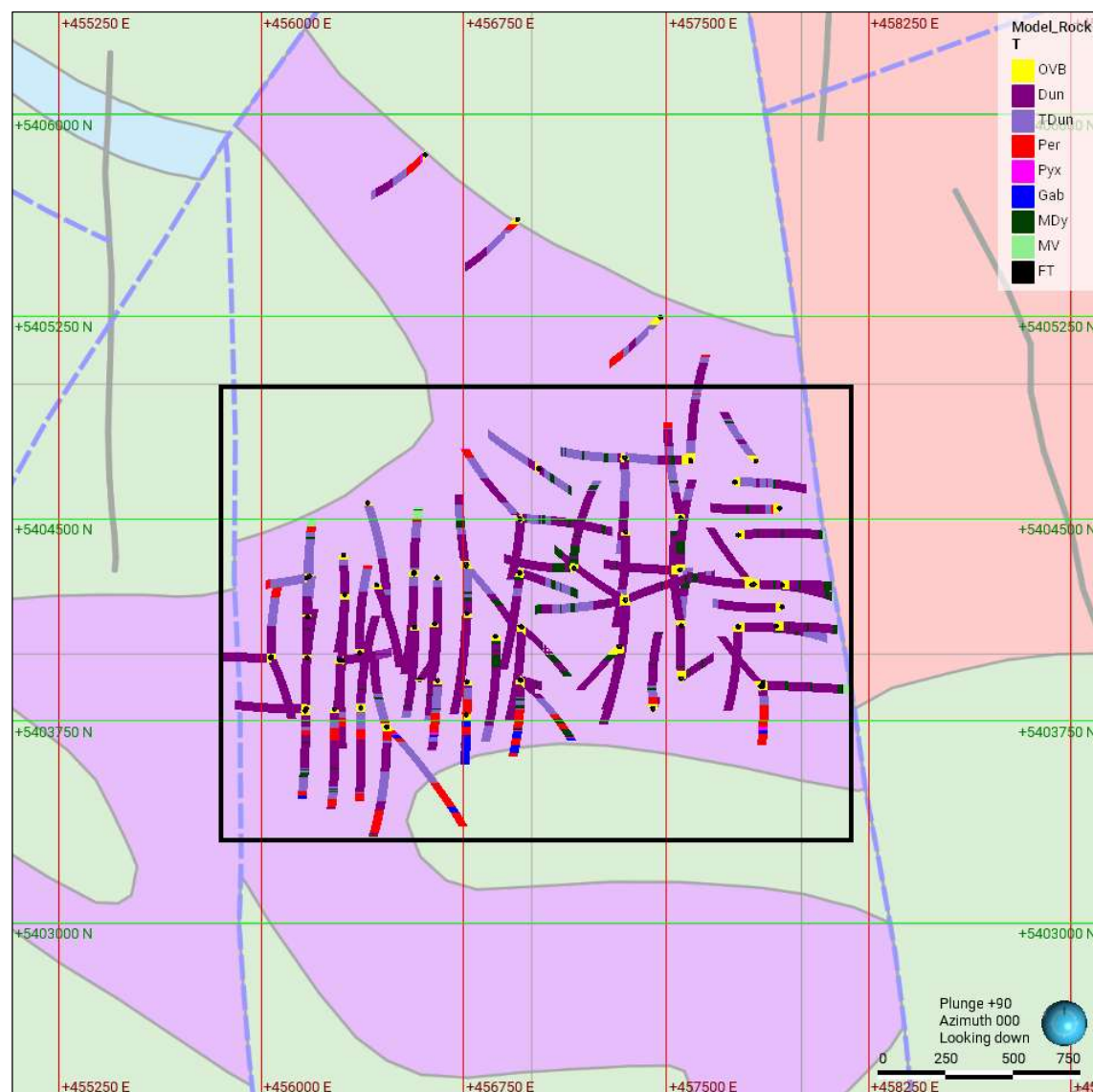
Figure 14-4. Plan view of the Reid Deposit with MRE drill hole intervals showing the final lithology codes for modelling. Background lithology from OGS (Ayer and Trowell, 1998). The black rectangle represents the resource boundary and main modelling area (Caracle Creek, 2026).
