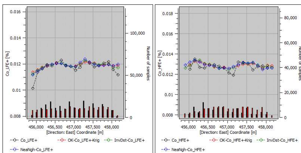
Figure 14-32. Cobalt swath plots for validation of the LFE (left) and HFE (right) domains (Caracle Creek, 2026).
