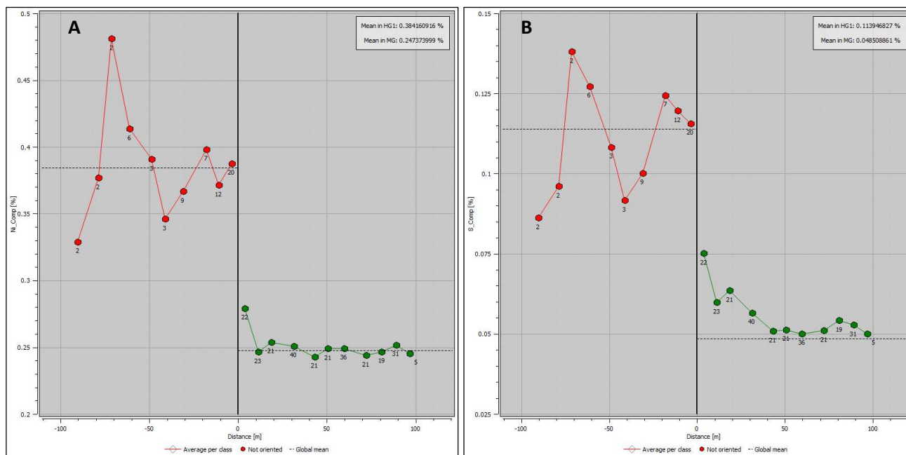
Figure 14-20. Contact analysis plots of: A) Nickel composites at the HG/MG domain boundary, B) Sulphur composites at the HG/MG domain boundary (Caracle Creek, 2026).
