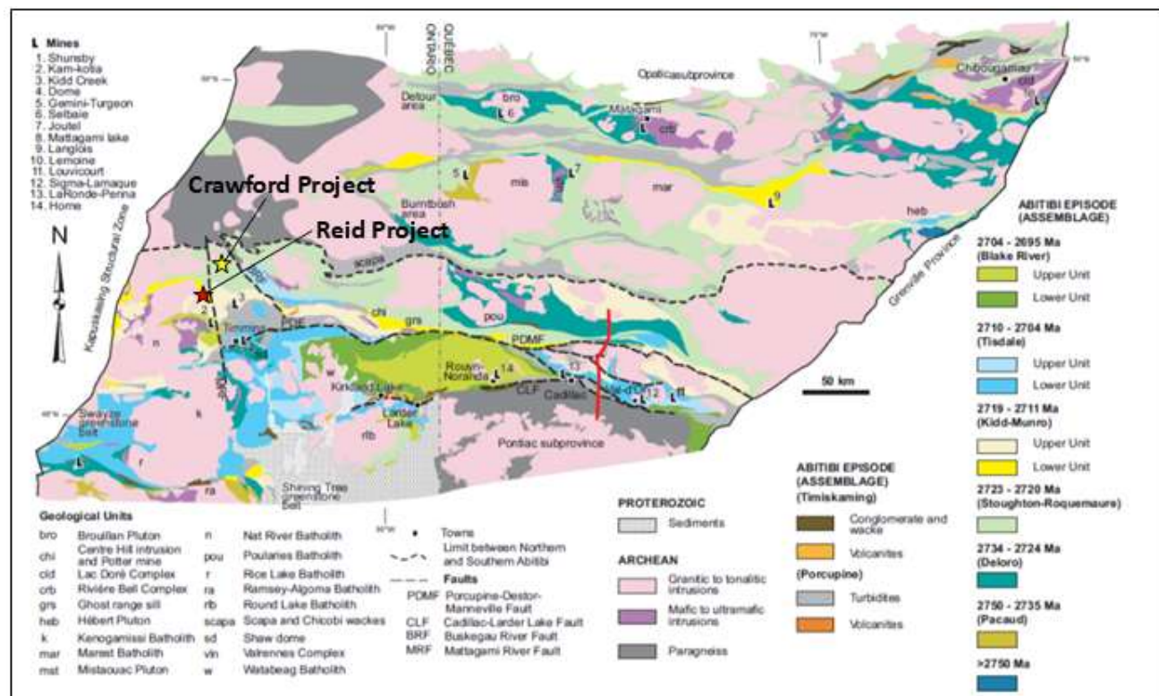
Figure 7-1. Regional geological setting of the Reid Nickel Sulphide Project (red star) area in the Abitibi Sub-province, Ontario. Also shown is the location of Canada Nickel's Crawford Nickel Property (yellow star) (after Thurston et al. , 2008).
