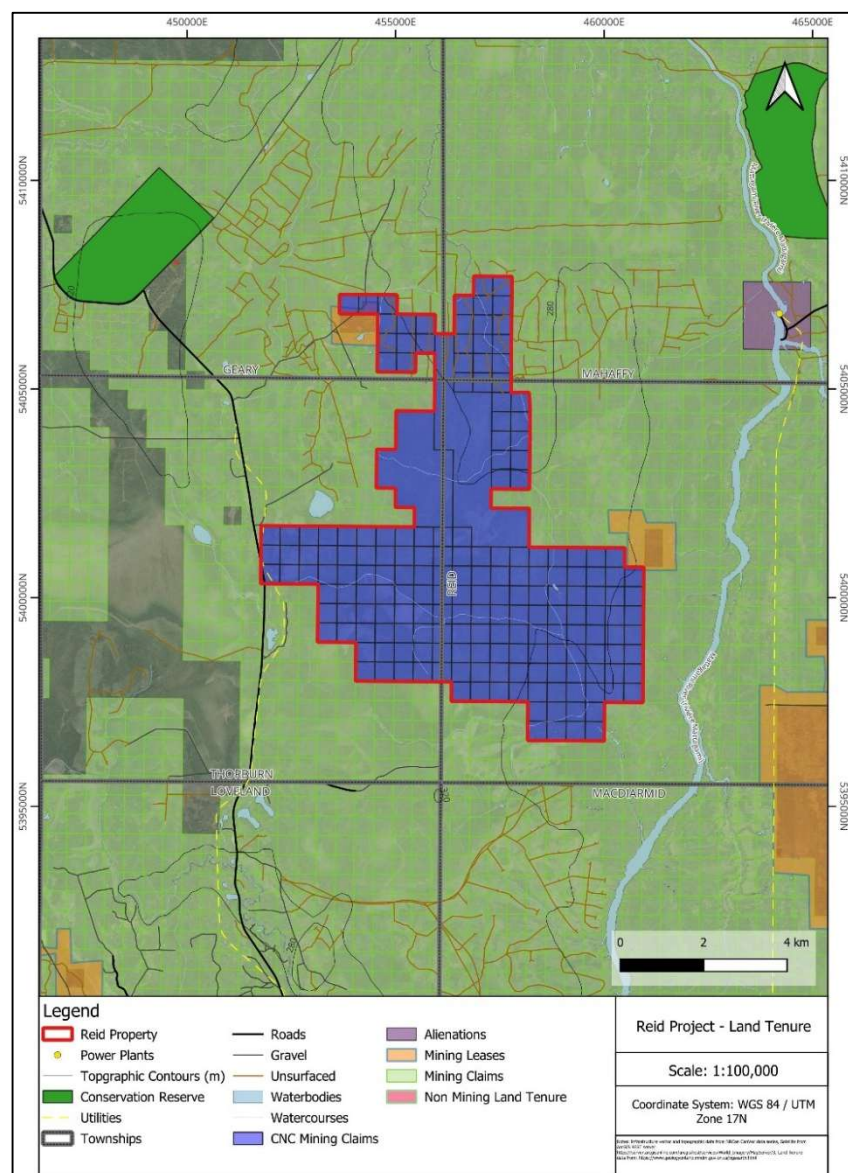
Figure 4-2. Township-scale map showing the location of the Reid Nickel Sulphide Project and surround mining lands (from MLAS, Government of Ontario, 2024; Caracle Creek, 2026).
