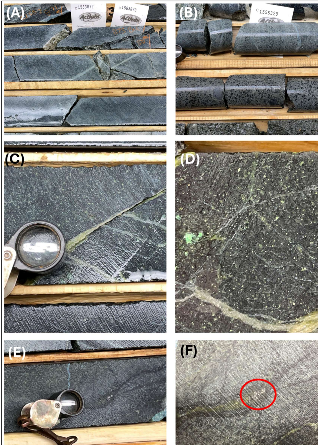
Figure 2-2. Photos taken during the Personal Inspection of the Reid Nickel Sulphide Project in February 2026, (A) Nondescript pyroxenite from hole REI-25-66 that carries up to 1.96 g total PGEs per tonne. (B) Similar pyroxenite from hole REI25-67 again carrying anomalous PGEs but low grades in Ni. This core has been cut using a mechanical hydraulic core splitter. (C) Oxidizing heazlewoodite (“nickel bloom”) in the core from hole REI25-69. Assays of up to 0.5% Ni are noted. (D) Close up of previous Figure C. (E) Fracture-controlled heazlewoodite from hole REI25-84. (F) Close up of previous Figure E (Caracle Creek, 2026).
