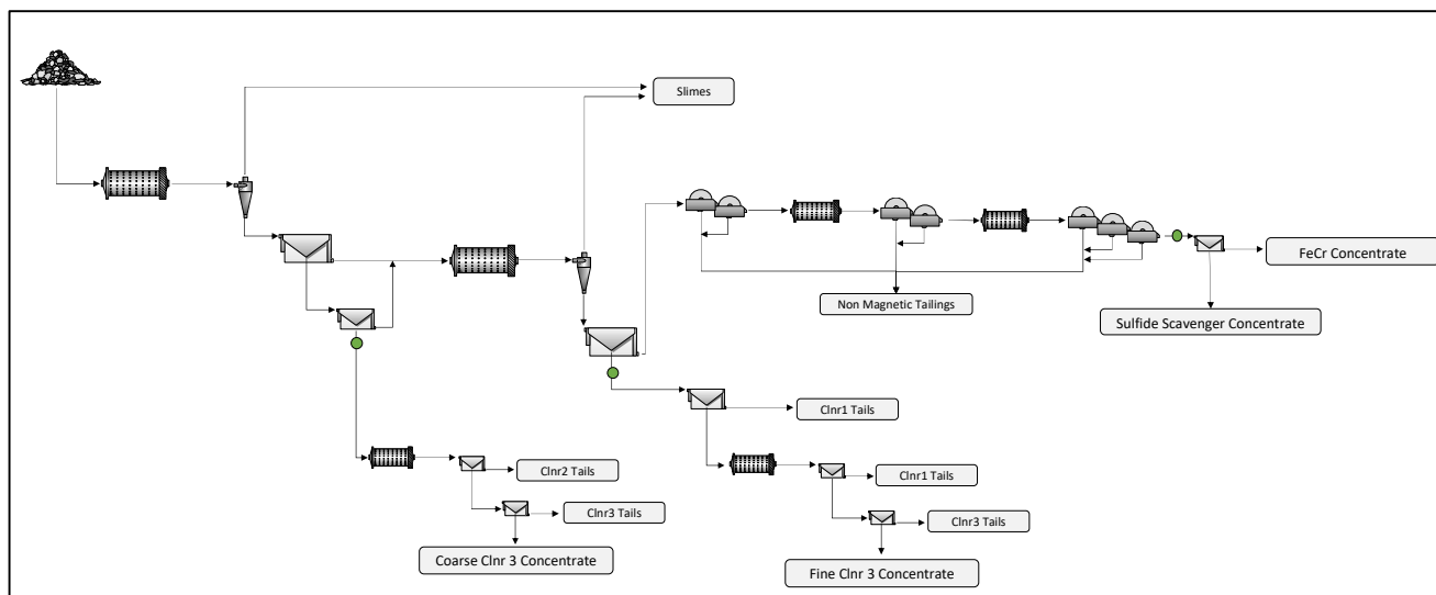
Figure 13-1. Open circuit test flowsheet (Canada Nickel, 2024).
