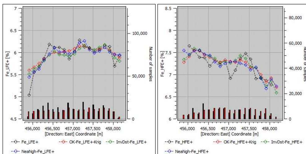
Figure 14-33. Iron swath plots for validation of the LFE (left) and HFE (right) domains (Caracle Creek, 2026).
