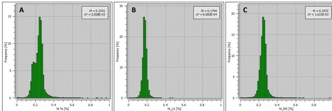
Figure 14-11. Nickel grade histograms within: A) EST Domain, B) LG Domain and C) MG domain (Caracle Creek, 2026).
