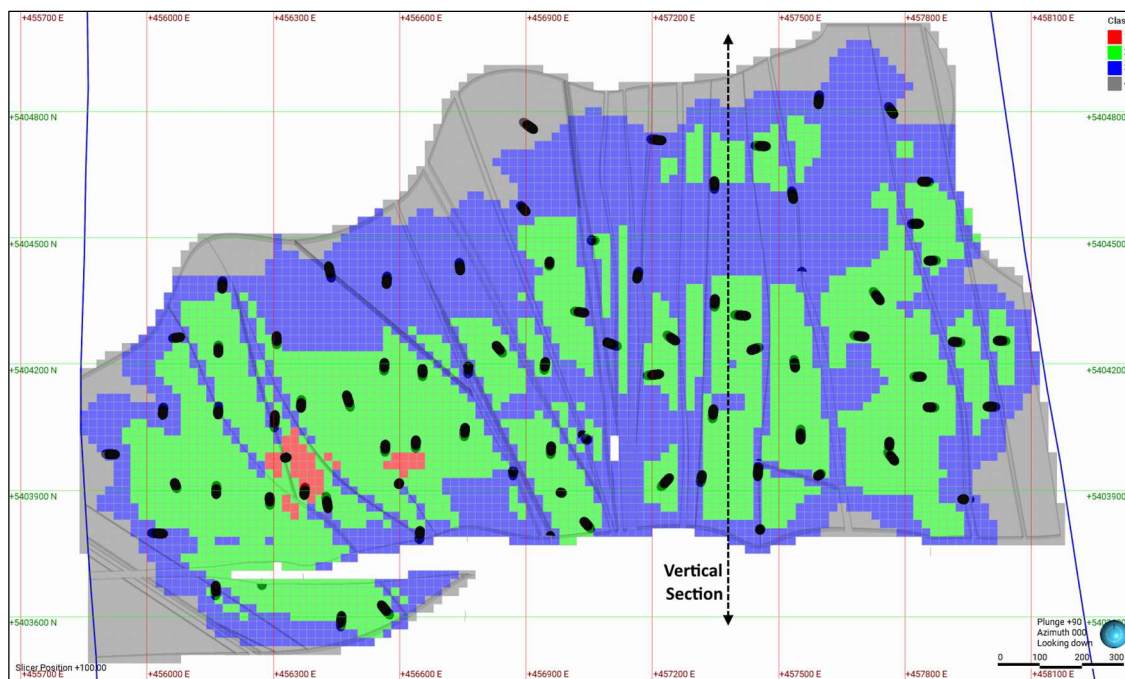
Figure 14-37. Plan section (RL 100) of the Reid resource classification against drill hole intercepts within the EST domain, and major faults (blue lines). Block colours represent measured (red), indicated (green) and inferred (blue) resource classes, as well as unclassified potential (grey). The dashed line is the trace of the vertical section presented in Figure 14-38 (Caracle Creek, 2026).
