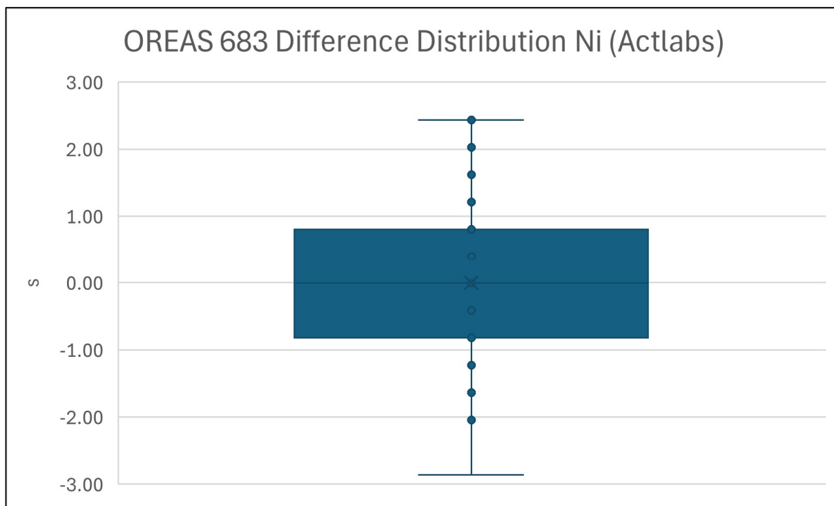
Figure 11-6. CRM OREAS 683 – Distribution of Standard Deviations Difference for Ni Analysis from the Average Value for Various Analytical Runs at Actlabs (Caracle Creek, 2026).
