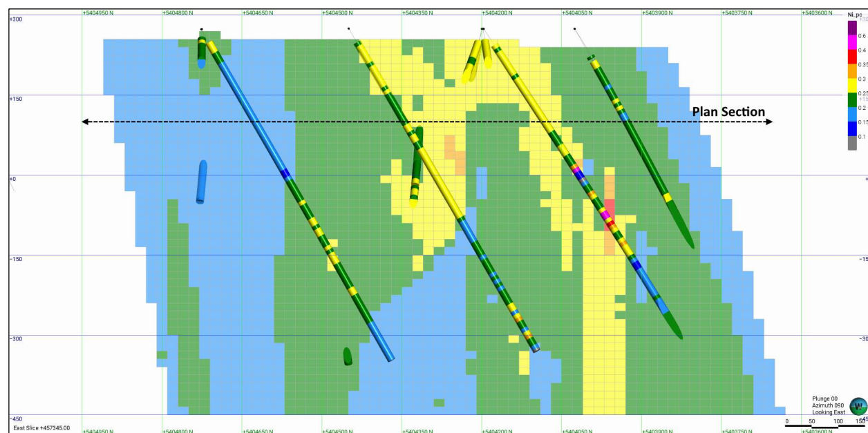
Figure 14-30. Vertical section 457,345 E (Looking East) of Reid nickel grade blocks against composites within the EST domain. Some intercepts may not precisely match their corresponding feature due to the 100 m section width. The dashed line is the trace of the plan section presented in Figure 14-29 (Caracle Creek, 2026).
