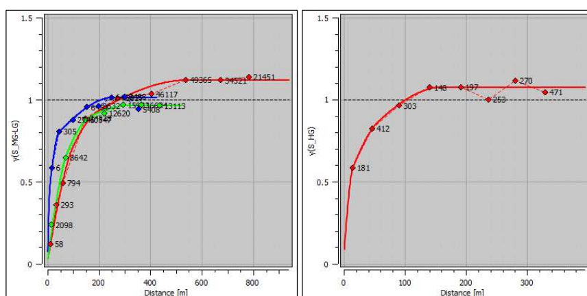
Figure 14-27. Sulphur variograms for the MG+LG (left) and HG (right) domains (Caracle Creek, 2026).
