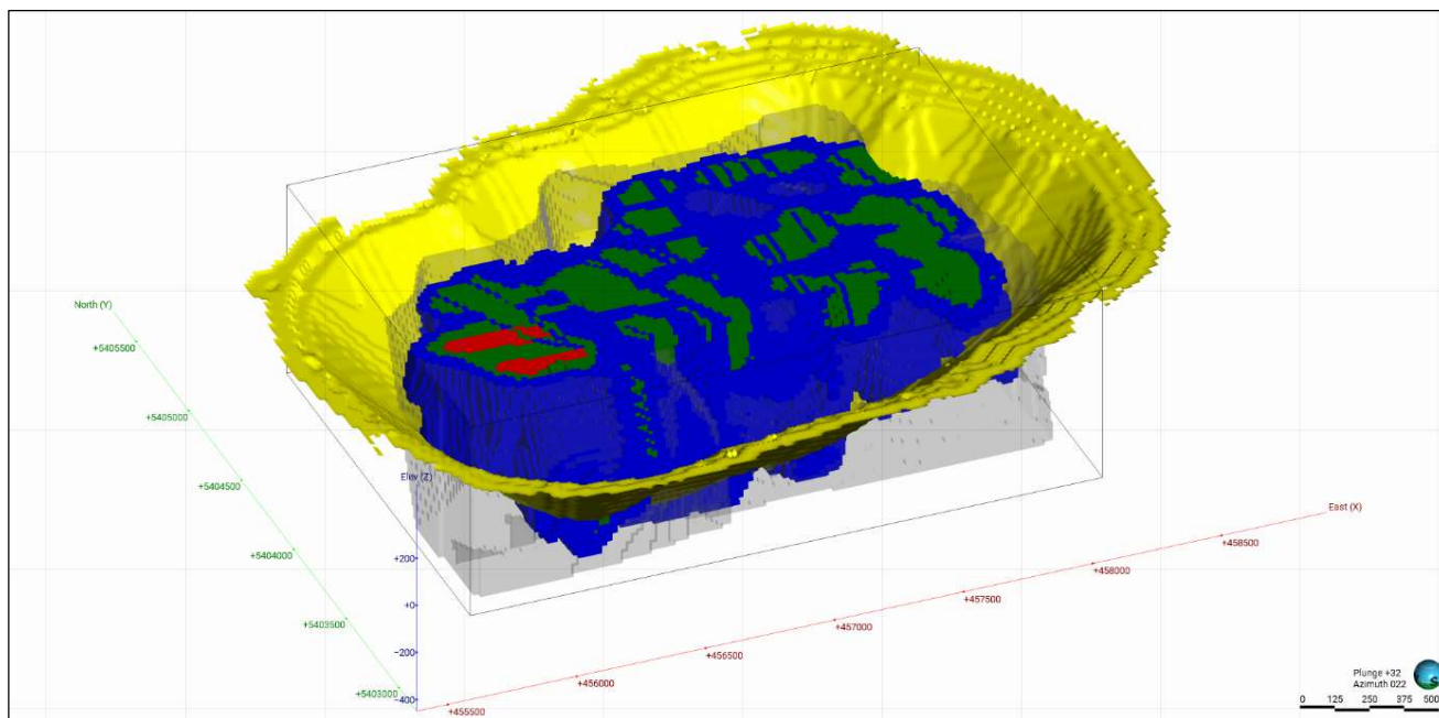
Figure 14-39. 3D Perspective (Looking Northeast) of the Reid Pit Shell (yellow) and Resource Class Blocks: Measured (red), Indicated (green), Inferred (blue) and unclassified potential (transparent grey). The box-shaped edges represent the current resource boundary and main modelling volume (Caracle Creek, 2026).
