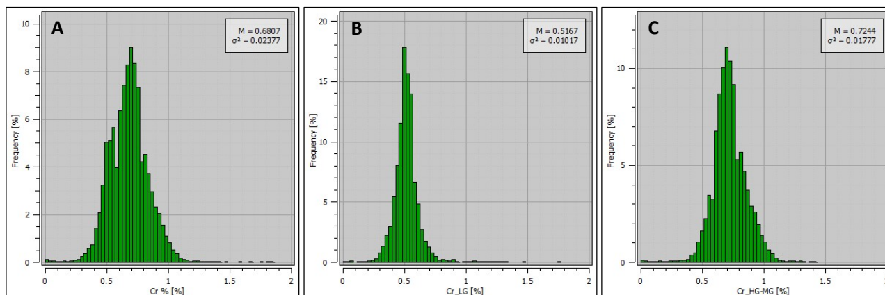
Figure 14-12. Chromium grade histograms within: A) EST Domain, B) LG Domain and C) MG+HG domain (Caracle Creek, 2026).
