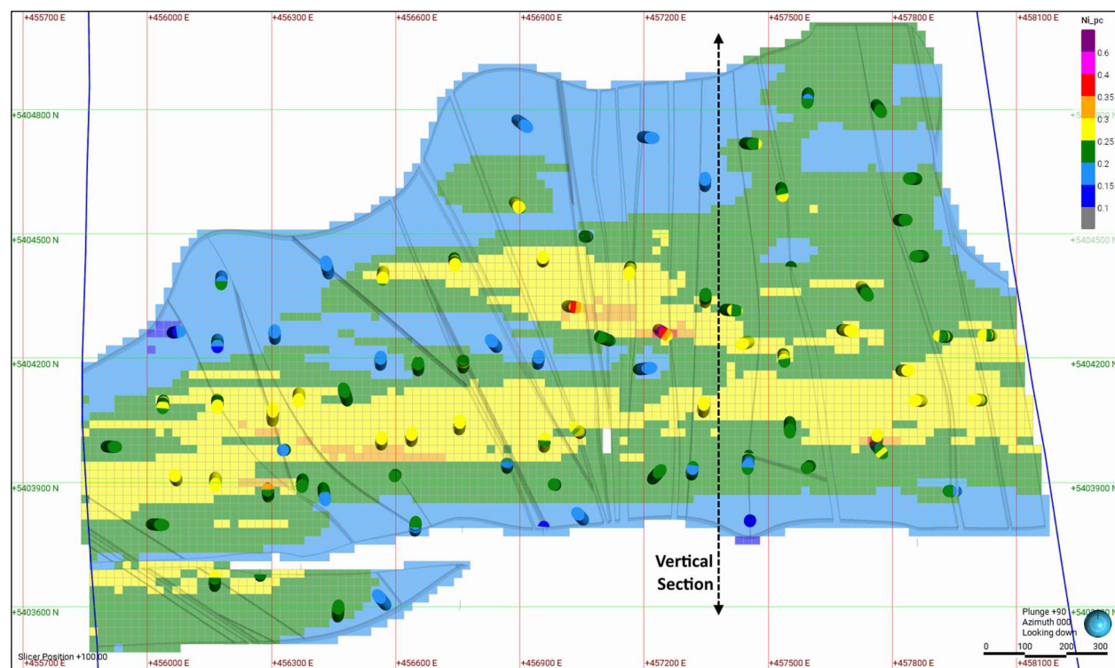
Figure 14-29. Plan section (RL 100) of Reid nickel grade blocks against composites within the EST domain, and major faults (blue lines). The dashed line is the trace of the vertical section presented in Figure 14-30 (Caracle Creek, 2026).
