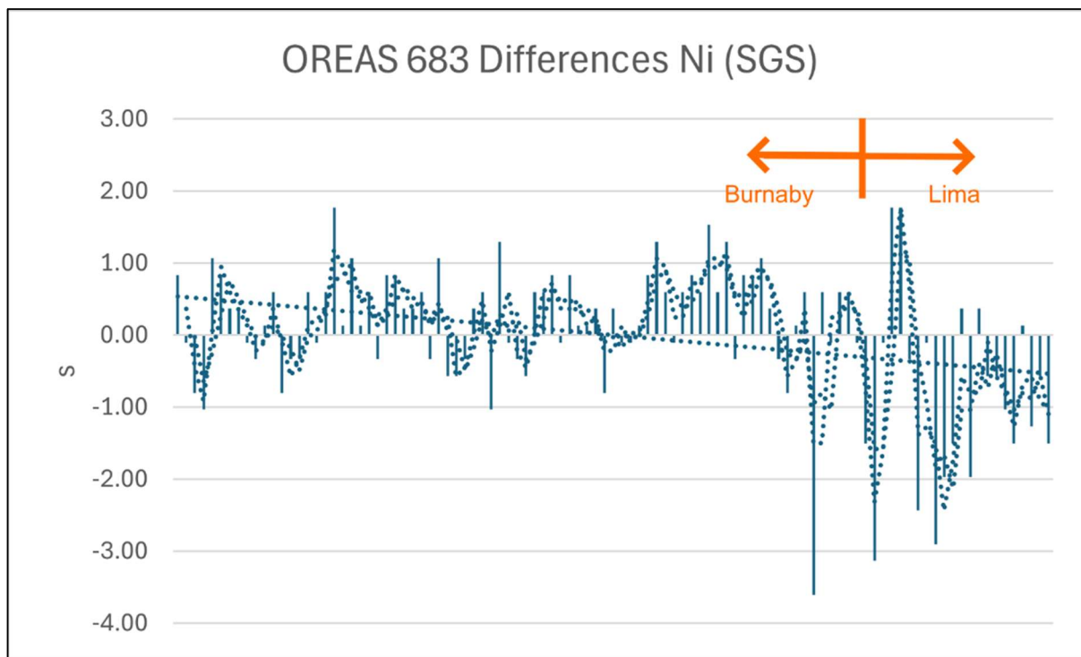
Figure 11-7. CRM OREAS 683 – Number of Standard Deviations Difference for Ni Analysis from the Average Value for Various Analytical Runs at SGS (Caracle Creek, 2026).
