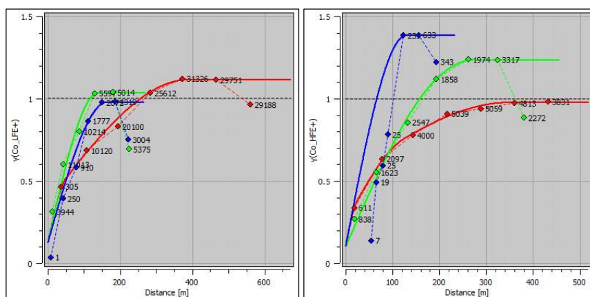
Figure 14-24. Cobalt variograms for the LFE (left) and HFE (right) domains (Caracle Creek, 2026).
