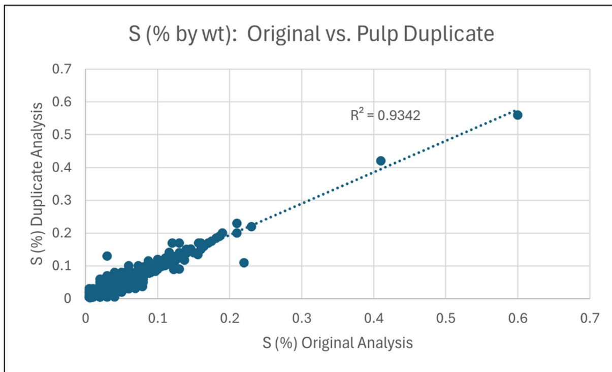
Figure 11-14. Plot of Absolute Concentrations of Pairs of Duplicate Samples Analyzed for S (Caracle Creek, 2026).
