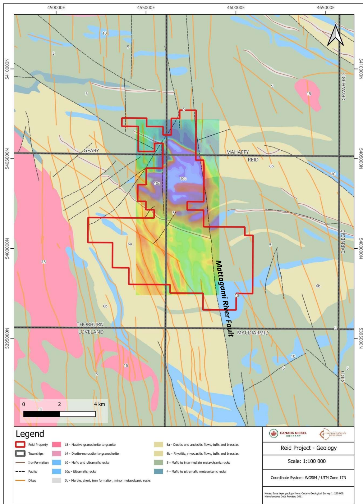
Figure 7-3. Township-scale generalized geological map (geological base from OGS) for the Reid Nickel Sulphide Project showing the outline of the mining claims boundary (red), the regional Mattagami River Fault, and where available, the total field (TF) magnetics (Caracle Creek, 2026).
