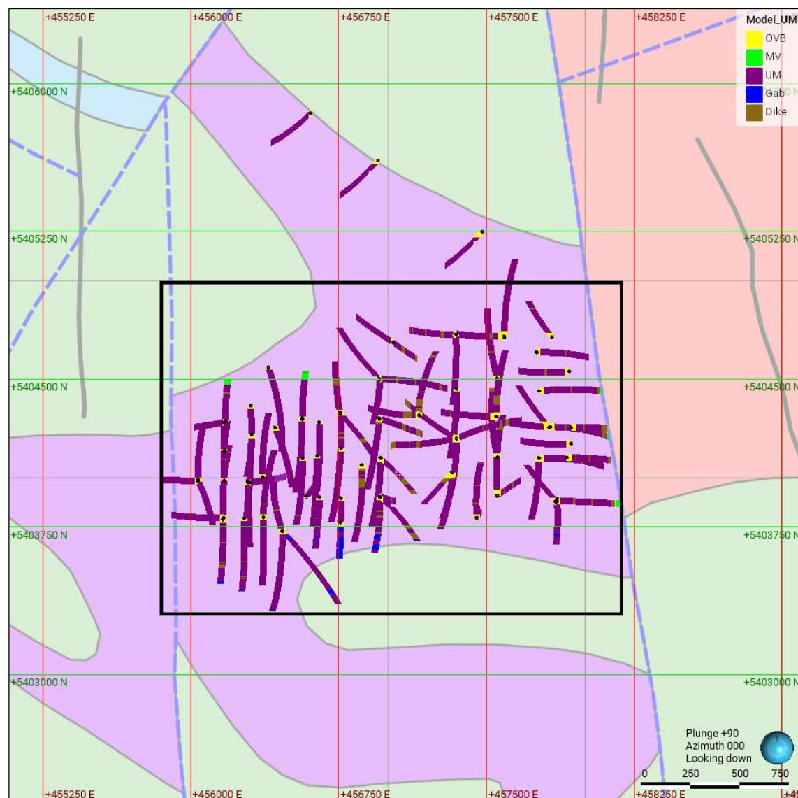
Figure 14-3. Plan view of the Reid Deposit with MRE drill hole intervals showing the main rock types. Background lithology from OGS (Ayer and Trowell, 1998). The UM package is coloured purple in the map and drill traces. The black rectangle represents the resource boundary and main modelling area (Caracle Creek, 2026).
