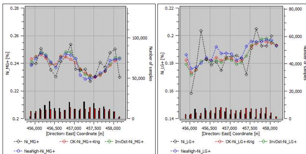
Figure 14-31. Nickel swath plots for validation of the MG (left) and LG (right) domains (Caracle Creek, 2026).
