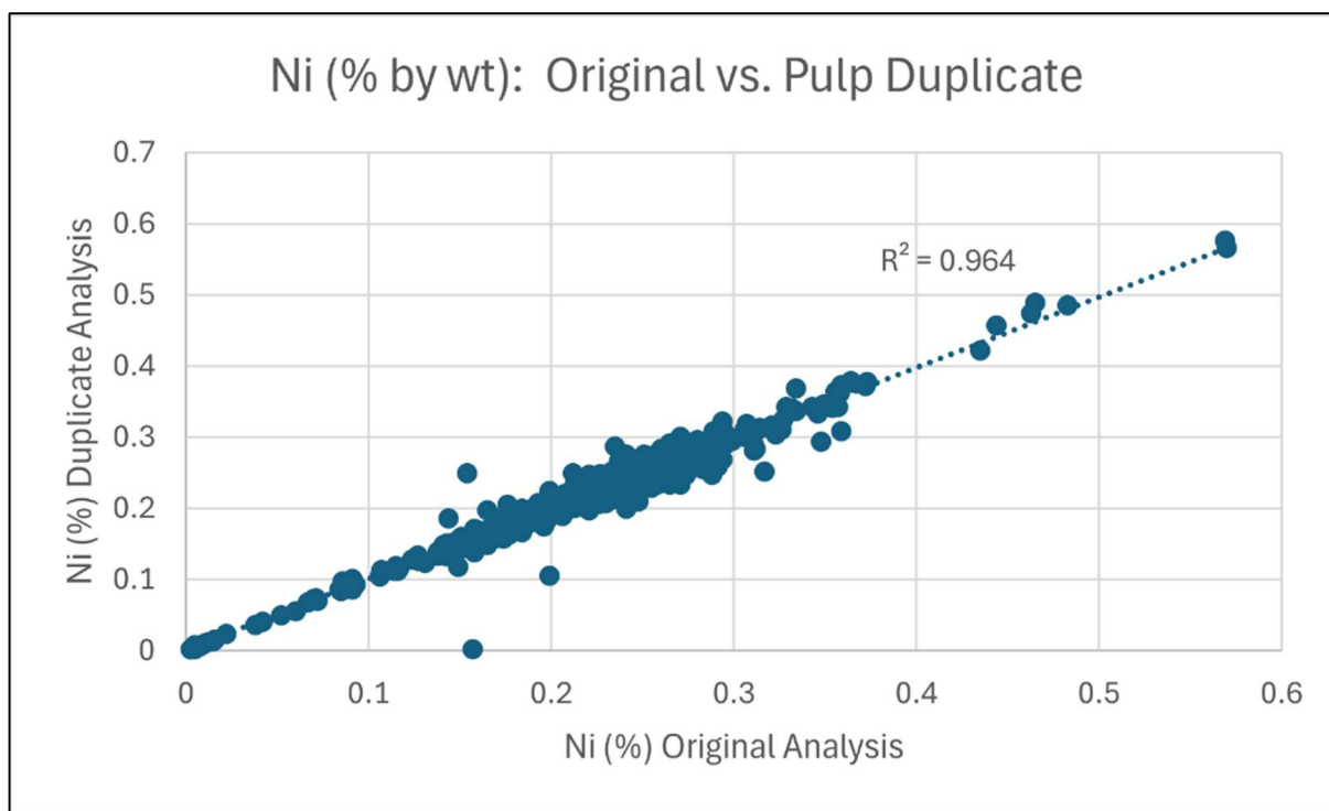
Figure 11-12. Plot of Absolute Concentrations of Pairs of Duplicate Samples Analyzed for Ni (Caracle Creek, 2026).
