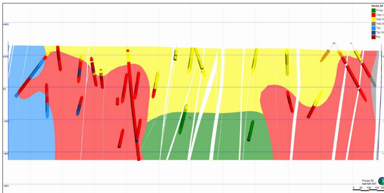
Figure 14-8. Oblique vertical section (Looking Northwest) of the Reid alteration model (limited to the dunite envelope), major faults (bounding blue lines) and coded drill hole intervals. Some drill hole intercepts may not precisely match their corresponding feature due to the 75 m section width (Caracle Creek, 2026).
