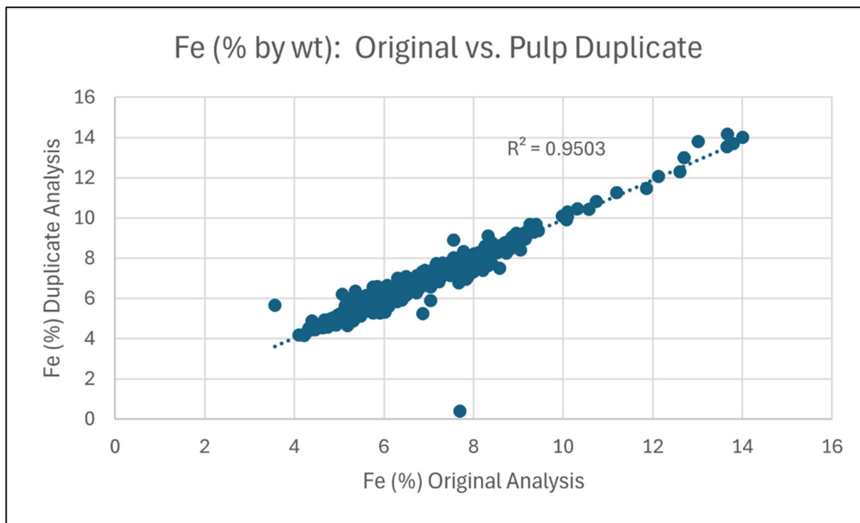
Figure 11-18. Plot of Absolute Concentrations of Pairs of Duplicate Samples Analyzed for Fe (Caracle Creek, 2026).
