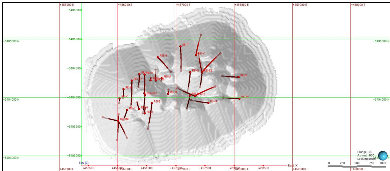
Figure 26-1. Plan map of the Reid Deposit showing the location of the MRE pit envelope and the planned drill hole projections (Caracle Creek, 2026).
