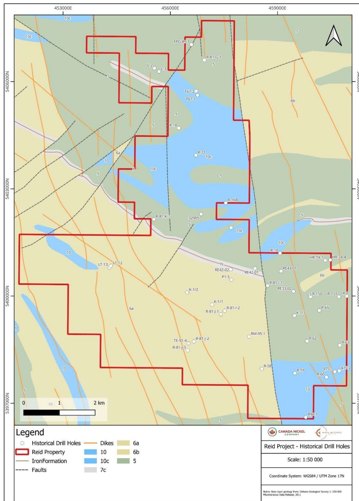
Figure 6-2. Location of all known historical drill holes (core and RC) within the Reid Project boundary (red) along with generalized geology (OGS). Table 6-2 provides a summary description of the historical drilling (Caracle Creek, 2026).
