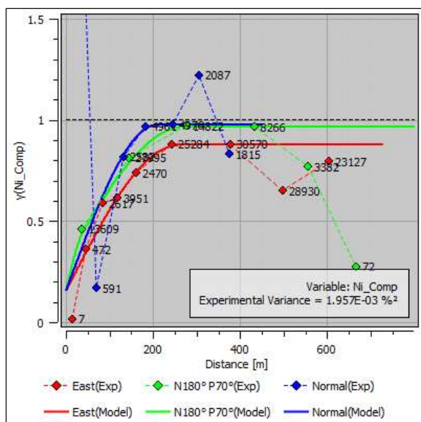
Figure 14-36. Variogram of nickel in the EST domain for resource classification (Caracle Creek, 2026).
