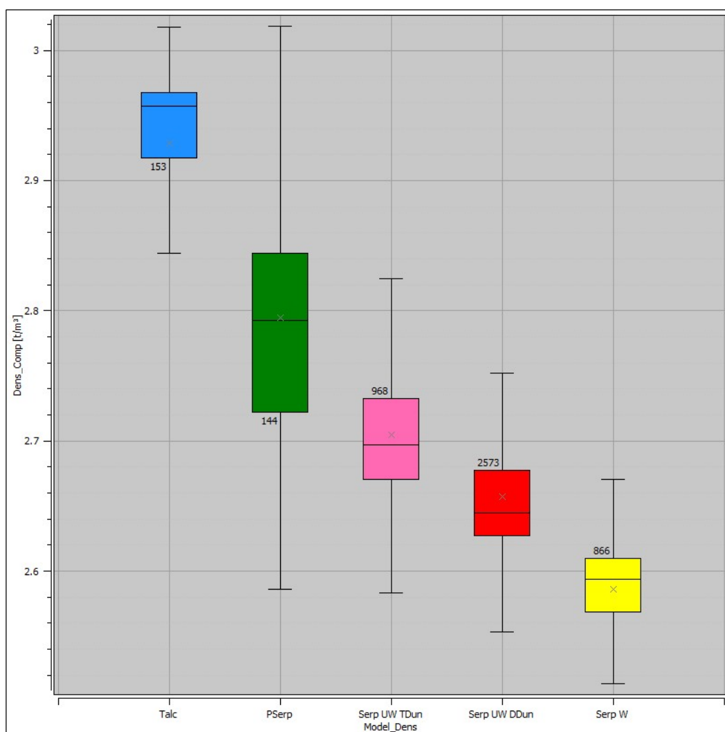
Figure 14-17. Boxplot of density values according to the alteration model and further subdivision of the Serp UW domain by dunite variant (Caracle Creek, 2026).
