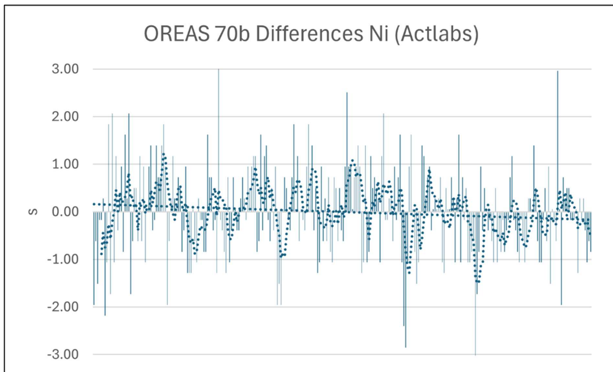
Figure 11-1. CRM OREAS 70b – Number of Standard Deviations Difference for Ni Analysis from the Average Value for Various Analytical Runs at Actlabs (Caracle Creek, 2026).
