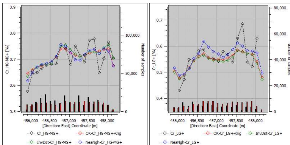
Figure 14-34. Chromium swath plots for validation of the HG+MG (left) and LG (right) domains (Caracle Creek, 2026).
