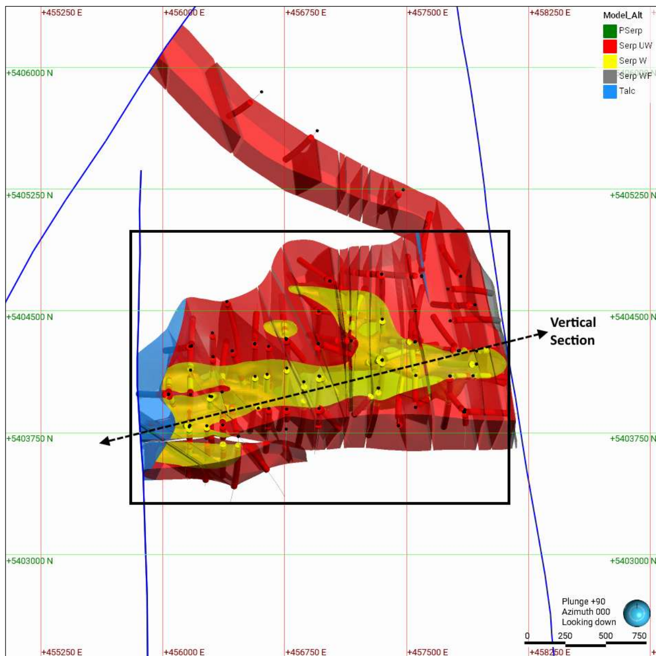
Figure 14-7. Plan view of the Reid alteration model (limited to the dunite envelope), major faults (blue lines) and coded drill hole intervals. The black rectangle represents the resource boundary and main modelling area, and the dashed line is the trace of the vertical section presented in Figure 14-8 (Caracle Creek, 2026).
