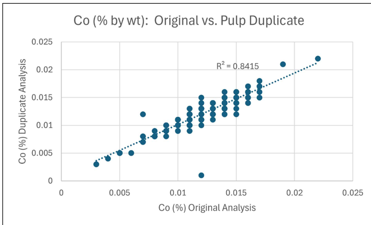
Figure 11-13. Plot of Absolute Concentrations of Pairs of Duplicate Samples Analyzed for Co (Caracle Creek, 2026).
