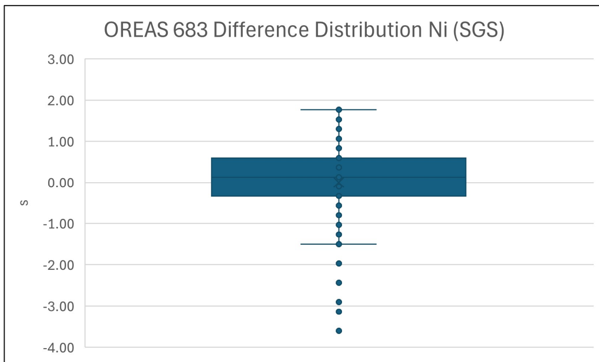
Figure 11-8. CRM OREAS 683 – Distribution of Standard Deviations Difference for Ni Analysis from the Average Value for Various Analytical Runs at SGS (Caracle Creek, 2026).
