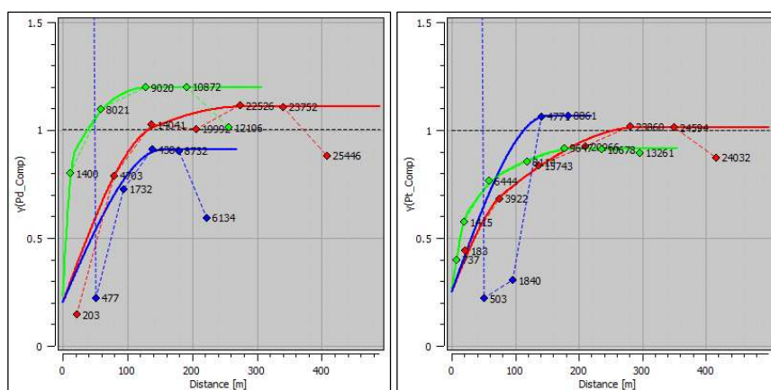
Figure 14-28. Variograms of palladium (left) and platinum (right) for the EST domain (Caracle Creek, 2026).
