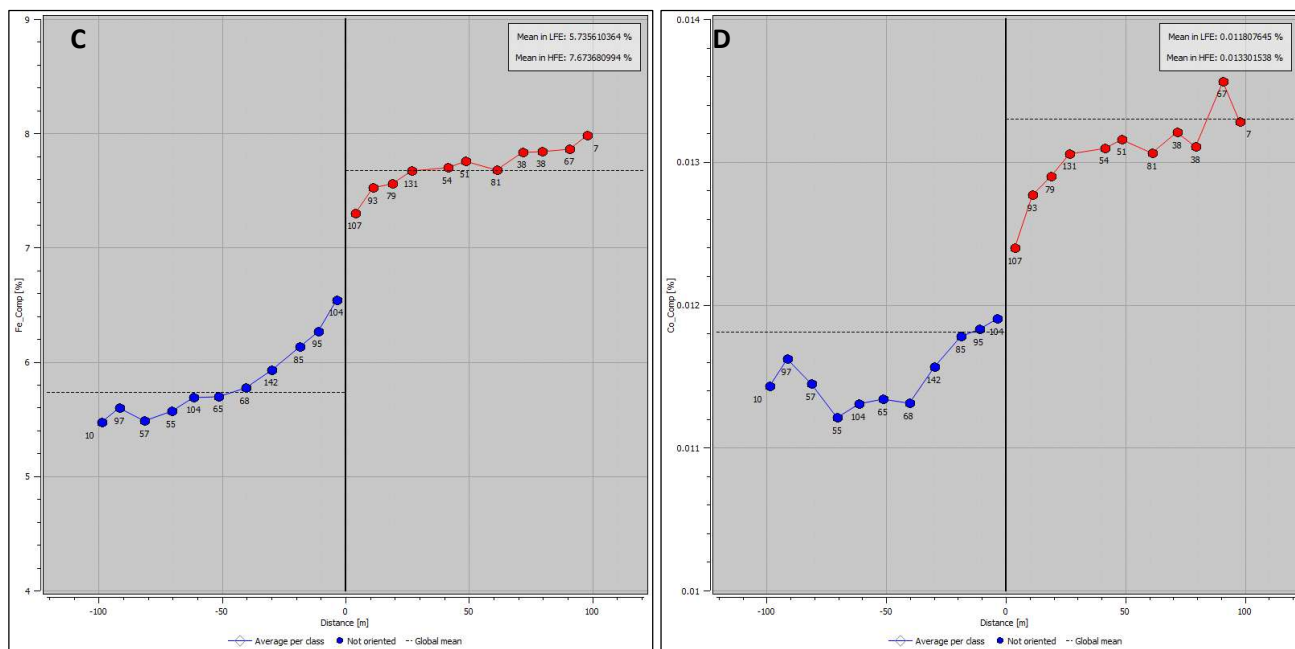
Figure 14-21. Contact analysis plots of: A) Nickel composites at the MG/LG domain boundary, B) Chromium composites at the MG/LG domain boundary, C) Iron composites at the LFE/HFE domain boundary and D) Cobalt composites at the LFE/HFE domain boundary (Caracle Creek, 2026).
