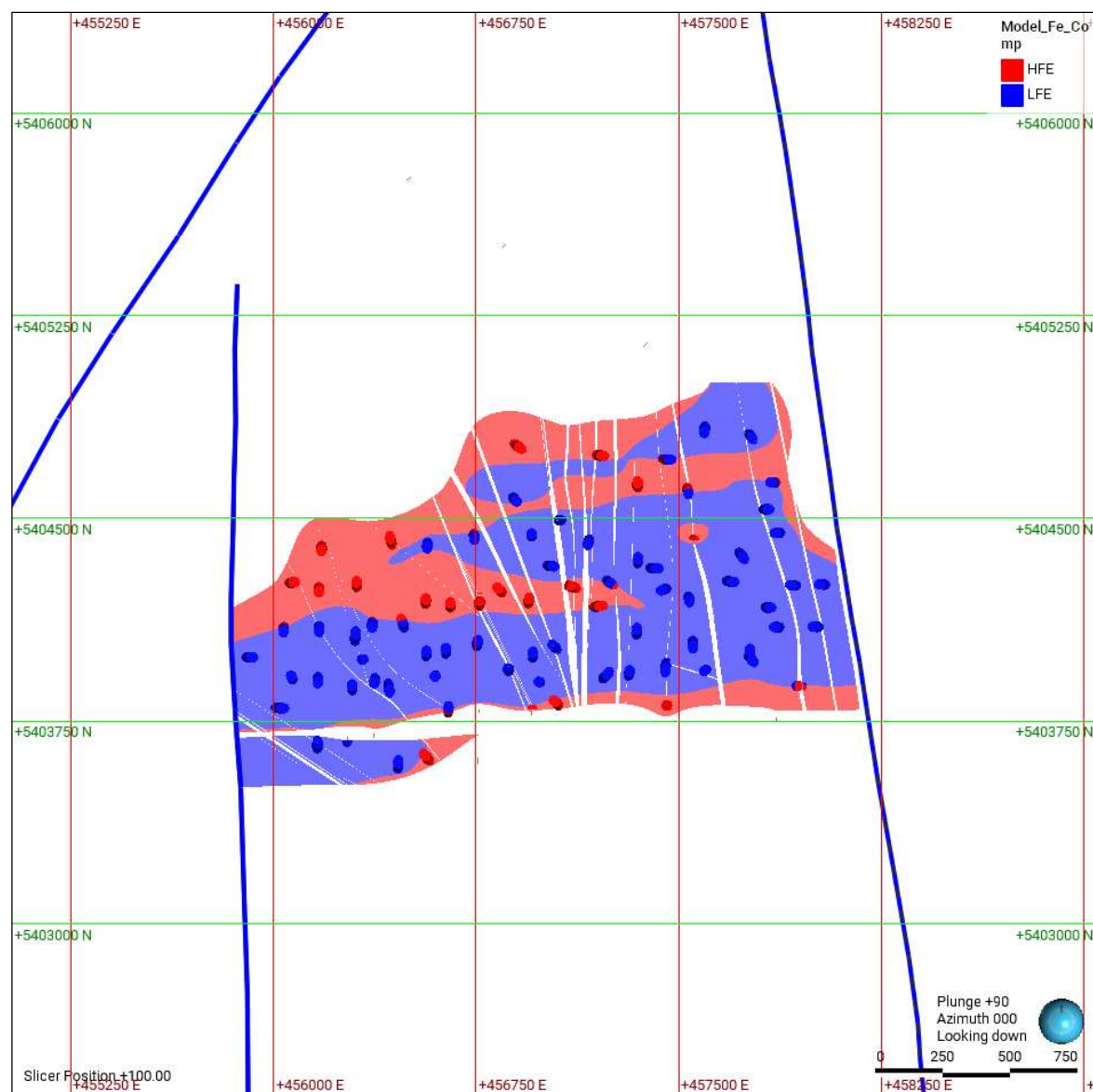
Figure 14-19. Plan section (RL 100) of the Reid iron/cobalt estimation domains, major faults (blue lines) and coded drill hole intervals. The HFE Domain ( >7.0\% Fe) is coloured red and the LFE Domain ( <7.0\% Fe) is coloured blue (Caracle Creek, 2026).
