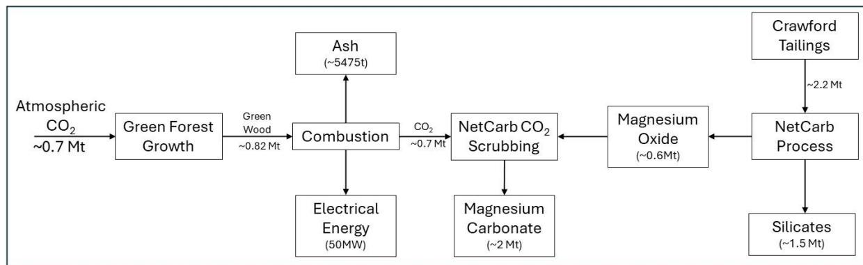
Figure 2b: 50MW power generation from forest and agricultural biomass co with carbon sequestration
