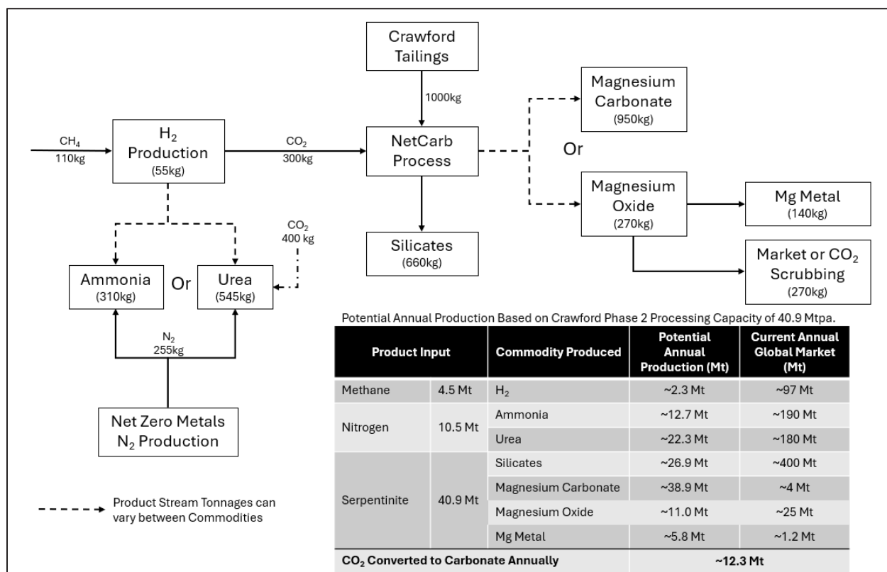
Figure 1: Hydrogen and Magnesium Products Generated per 1 tonne and annual volume of Crawford tailings
